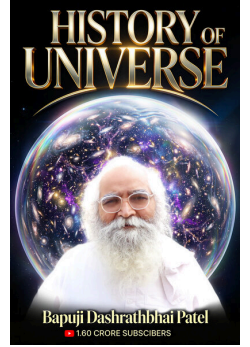
History of Universe
